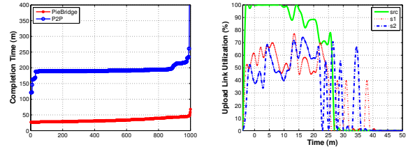
(a) Completion time.
